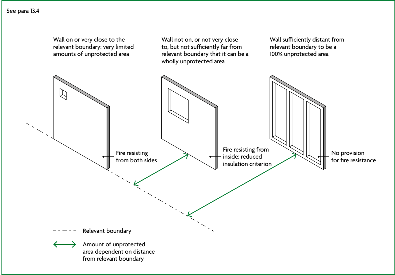
Diagram 13.1 Principles of space separation
